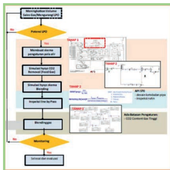
Gambar 13. Diagram Alir Sistem Blending Gas
