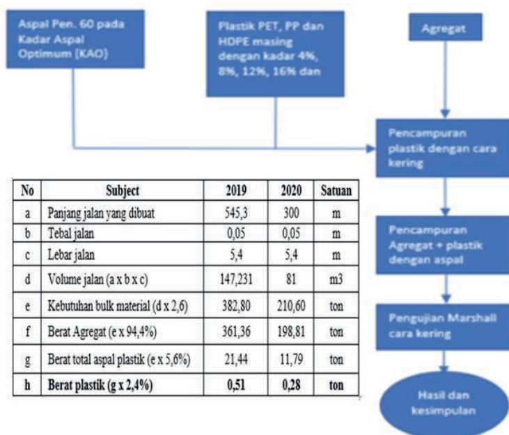
Gambar 90. Skema Inovasi Upgraded Asphalt Marshal Stability With PHP Plastik
