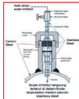
Gambar 85. Diagram Sistem TEE LESS
